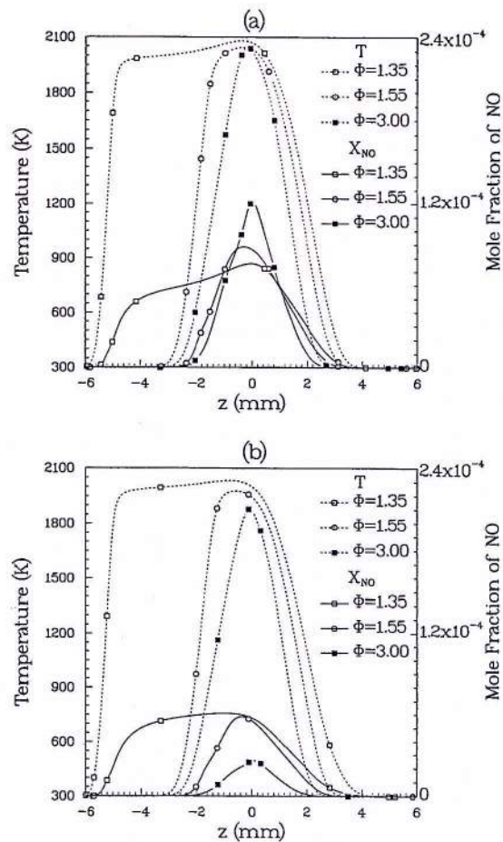
Predicted profiles of temperature and \text{NO} concentration in two-stage methane-air flames at different equivalence ratios \Phi : (a) without water; (b) with 10% water added in the air stream.
